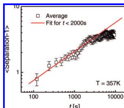
Figure 7. Log–log plot of the average time-dependent separation of hydroxyl pairs formed by water adsorption and dissociation on BBO_V 's at 357 K. The separation is plotted after the subtraction of initial offset of one lattice constant which represents the initial separation of geminate hydroxyl pairs. The linear fit for t < 2000 s has a slope of 0.45, very close to 0.5 expected for an ideal one-dimension random walk (see text, eq 6).
