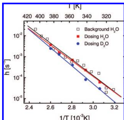
Figure 8. Arrhenius plot for along-row diffusion of hydrogen and deuterium for separated hydroxyl groups. The hydroxylated surfaces were prepared using dosed (red) and background (black) H 2 O and dosed (blue) D 2 O, on TiO 2 (110) at 300 K. The best fits to the data are shown with solid lines and yield the prefactors of 10^{7.6 \pm 0.6} , 10^{7.3 \pm 0.4} , and 10^{8.6 \pm 0.6} s -1 and diffusion barriers of 0.76 \pm 0.06 , 0.74 \pm 0.03 , and 0.85 \pm 0.04 eV for background H 2 O (black), dosed H 2 O (red), and dosed D 2 O (blue), respectively.
