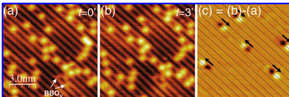
Figure 5. (a, b) Two subsequent ( \Delta t = 180 s) STM images (bias voltage: 1.5 V, tunneling current: 0.1 nA) on hydroxyl covered TiO_2(110) at 381 K illustrating the intrinsic diffusion of hydrogen along the BBO_V rows. The white arrows in (a) mark the positions of two remaining BBO_V 's. (c) Difference image, in which (a) is subtracted from (b); the dark (bright) spots represent the initial (final) hydrogen positions. The black arrows show the hopping directions. The black dotted lines mark the positions of the BBO_V rows.
